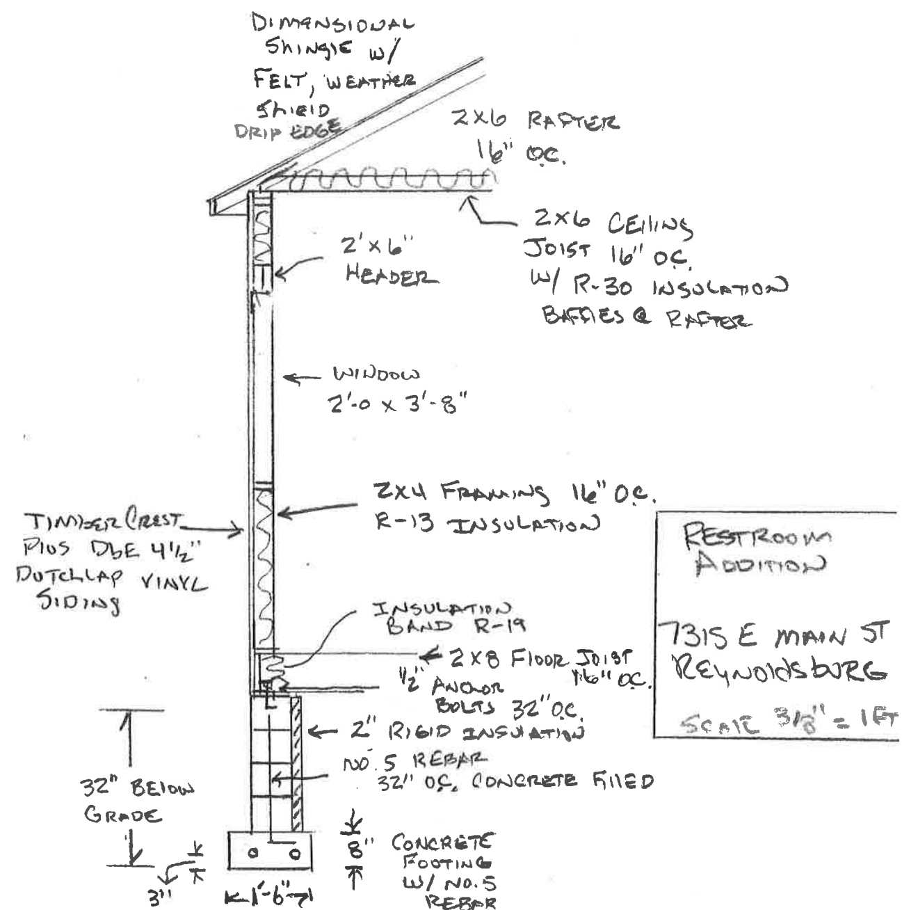
WALL SECTION
