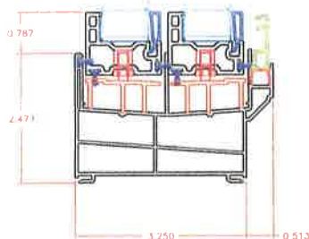
ThermalWeld SL Vertical Section
