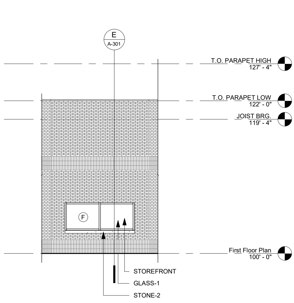
F Northeast Elevation Scale: 1/8" = 1'-0"
